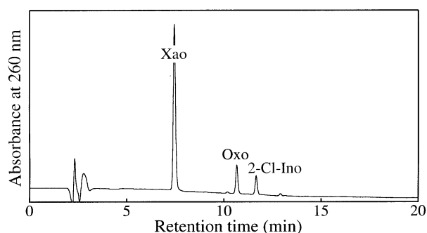
Figure 4. RP-HPLC chromatogram for the reaction mixture of the diazoate derivative of Guo incubated in the presence of NaCl. The RP-HPLC fraction containing the diazoate (20 \mu\text{L} ) was directly dropped into 2.5 M NaCl solution (80 \mu\text{L} ) containing 500 mM phosphate buffer (pH 7.4) and incubated at 37°C for 1 h. RP-HPLC conditions were the same as those described in Figure 1.
