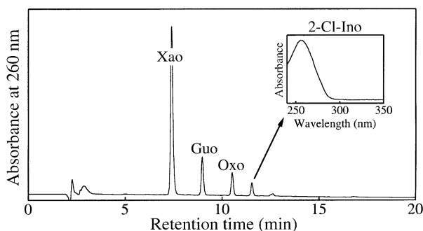
Figure 1. RP-HPLC chromatogram for the reaction mixture of Guo treated by \text{HNO}_2 in the presence of NaCl. Guo (1 mM) was incubated with 100 mM \text{NaNO}_2 and 2 M NaCl in 3 M sodium acetate buffer at pH 3.2 and 37 °C for 2 h. An HPLC system equipped with an ODS column (4.6×150 mm) was used. The eluent was 100 mM triethylammonium acetate (TEAA) buffer (pH 7.0) containing \text{CH}_3\text{CN} and the flow rate was 1 mL/min. The \text{CH}_3\text{CN} concentration was increased from 0 to 20% for 20 min in a linear gradient mode. Inset is an on-line detected UV spectrum of 2-Cl-Ino.
