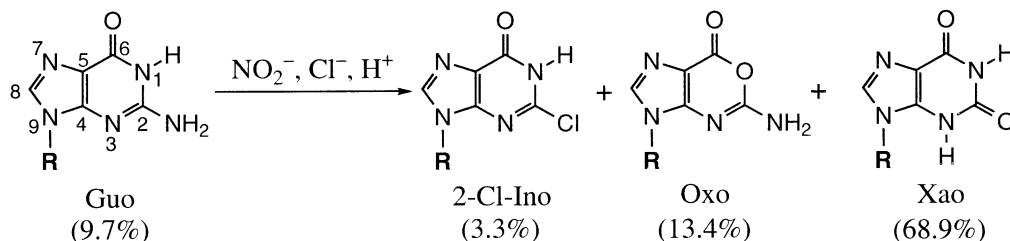
Figure 2. Reaction products of Guo treated by \text{HNO}_2 in the presence of NaCl. The numbers in the parentheses denote percentage yields of products at the reaction time of 2 h. R = ribose.
