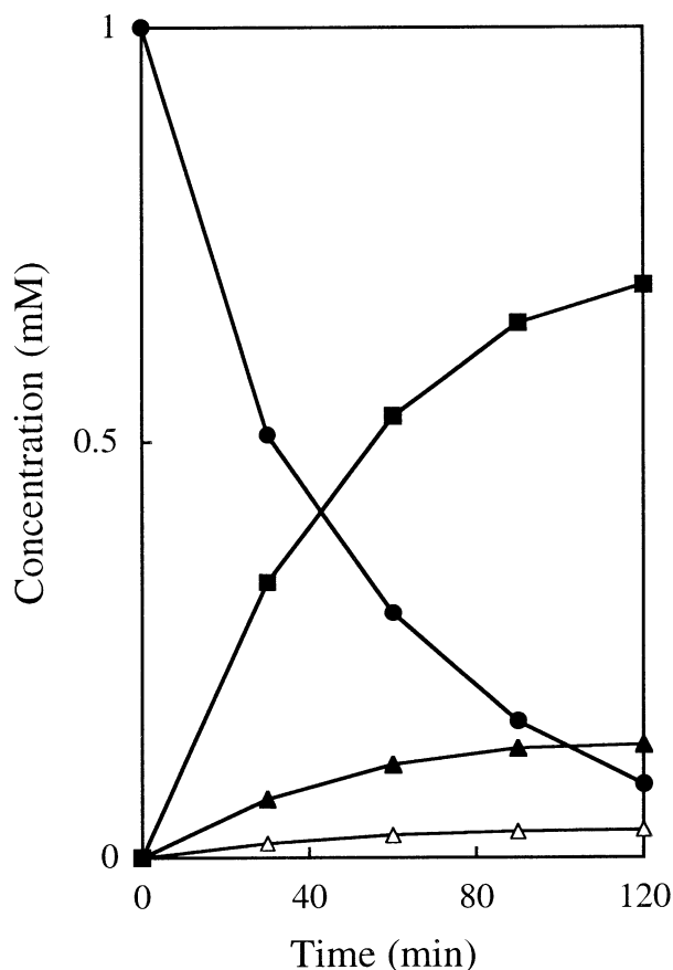
Figure 3. The time courses of formation of 2-Cl-Ino (open triangle), Oxo (closed triangle), Xao (closed square) and conversion of Guo (closed circle) when Guo (1 mM) was incubated with 100 mM \text{NaNO}_2 and 2 M NaCl in 3 M sodium acetate buffer at pH 3.2 and 37°C. The concentration was determined by RP-HPLC analysis.
