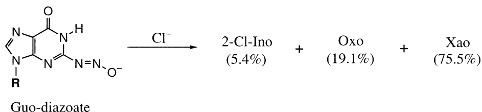
Figure 5. Reaction products formed from the diazoate derivative of Guo (Guo-diazoate) in the presence of NaCl. The numbers in the parentheses denote relative yields of products.
